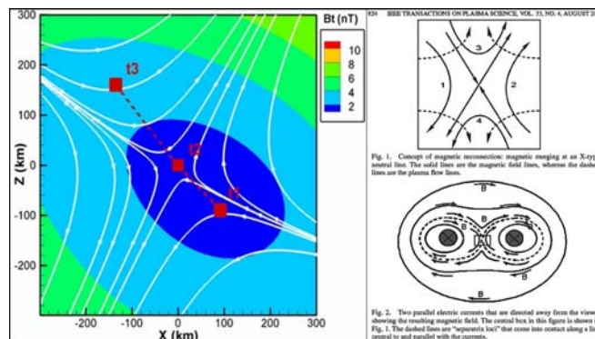
Fig. 2. Left: Magnetic field lines around a magnetic null observed by Cluster. Image credit: He, J.-S., et al. Right: Figs. 1 & 2 from Real Properties of Magnetic Fields in the Cosmos [7]. Image credit: Don Scott.
