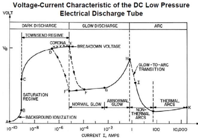
Fig. 1. Discharges are distinguished not only by their luminescence but also by their Current-Voltage characteristics, the current density and breakdown voltage. [5]
